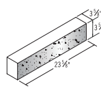
4x4x24 1F Solid
