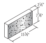
2 1/4 x 8 x 16 1F Solid
