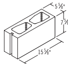
6x8x16 Sash
