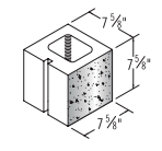
8x8x8 1F Half*
