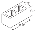
8x8x16 Regular
