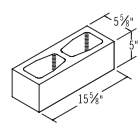
6x5x16 Starter
