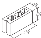
6x8x16 Knock-Out Deep Lintel
