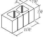
8x8x16 3-Score
