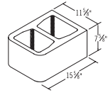
12x8x16 Double Bullnose
