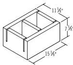
12x8x16 Knock-Out Bond Beam
