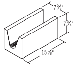
8x8x16 Solid Bottom Bond Beam
