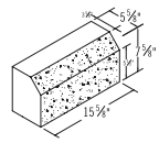
6x8x16 GF Chamfer
