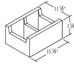
12x8x16 RS Bond Beam
