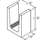
12x16x8 Deep Lintel Bond Beam
