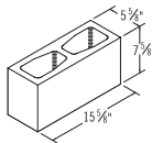
6x8x16 Regular
