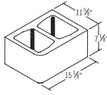
12x8x16 Single Bullnose
