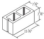
8x8x16 Sash
