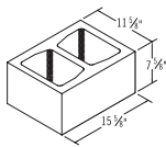
12x8x16 Regular
