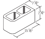
8x8x16 DBN
