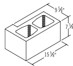
10x8x16 L Corner
