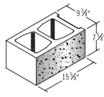
10x8x16 One Face
