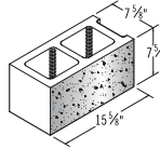
8x8x16 One Face
