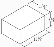
12x8x16 Solid
