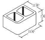
12x8x16 DBN Pillar
