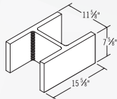
12x8x16 H Block
