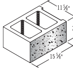
12x8x16 One Face
