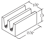
10x8x16 Solid Bottom Bond Beam
