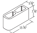
6x8x16 DBN
