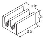
12x8x16 Solid Bottom Bond Beam
