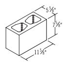
6x8x12 Three Quarter
