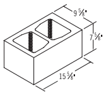
10x8x16 Regular
