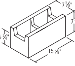
8x8x16 RS Bond Beam
