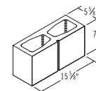
6x8x16 1-Score
