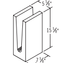
6x16x8 Deep Lintel Bond Beam
