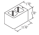
8x8x12 SBN Three Quarter
