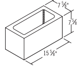
8x8x16 Single Core
