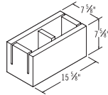
8x8x16 Knock Out Bond Beam
