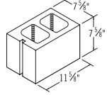
8x8x12 Three Quarter
